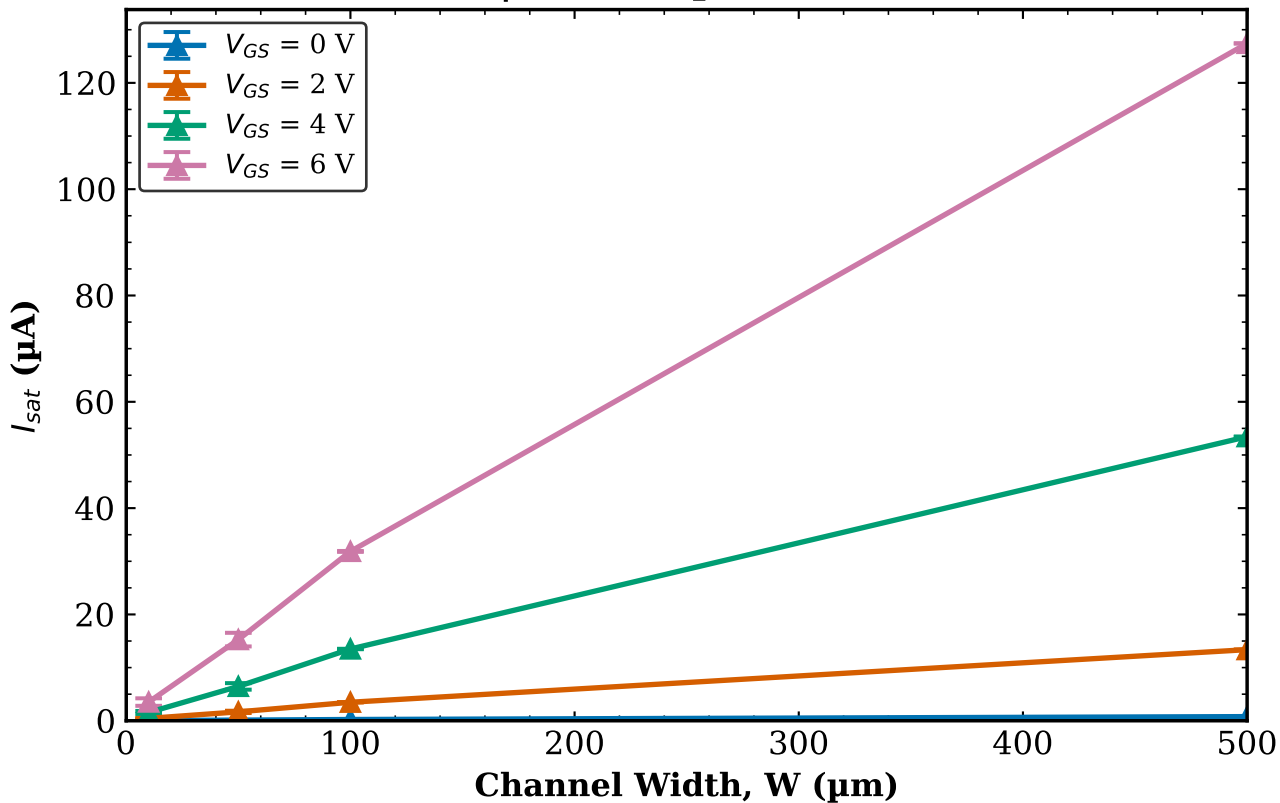
TFT1 Combined (Tr. 1 & 2) I_{sat} vs W | L = 40\text{ }\mu\text{m} (mean \pm std)
